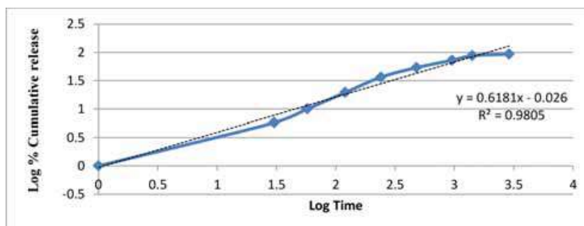
Figure 12: Peppas model release kinetics plot.
