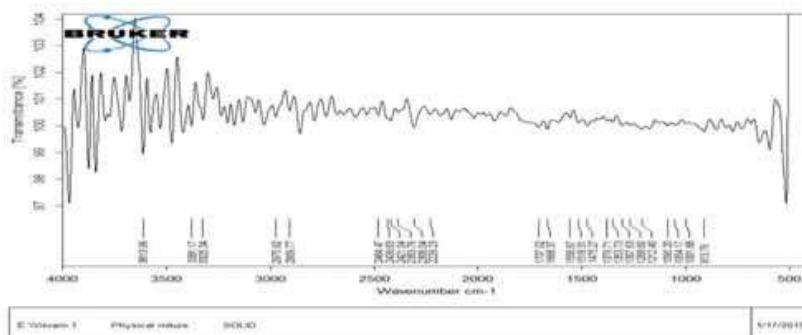
Figure 3: FTIR of Physical mixture.
