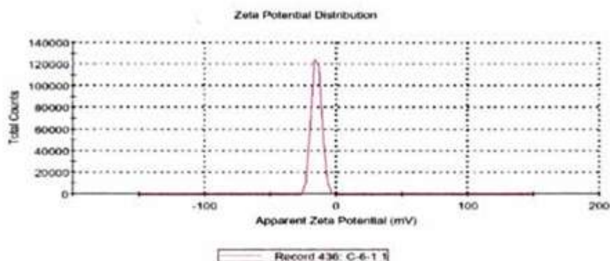
Figure 6: Zeta potential Copper nanoparticles
