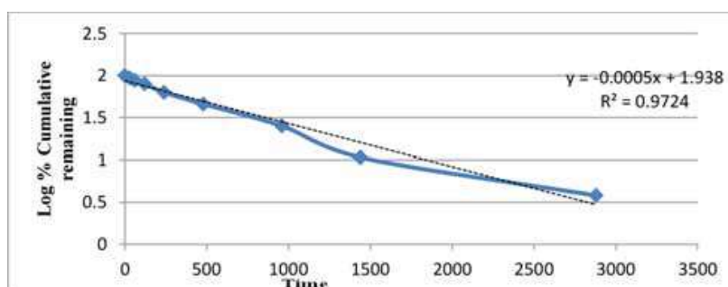
Figure 10: First Order release kinetics Plot.
