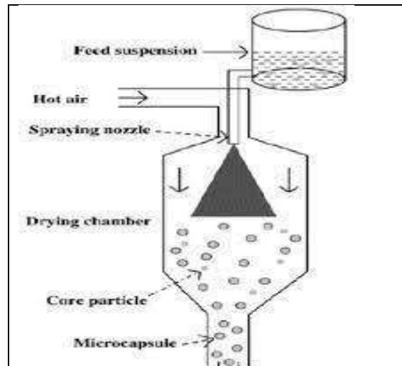
Air suspension coating
