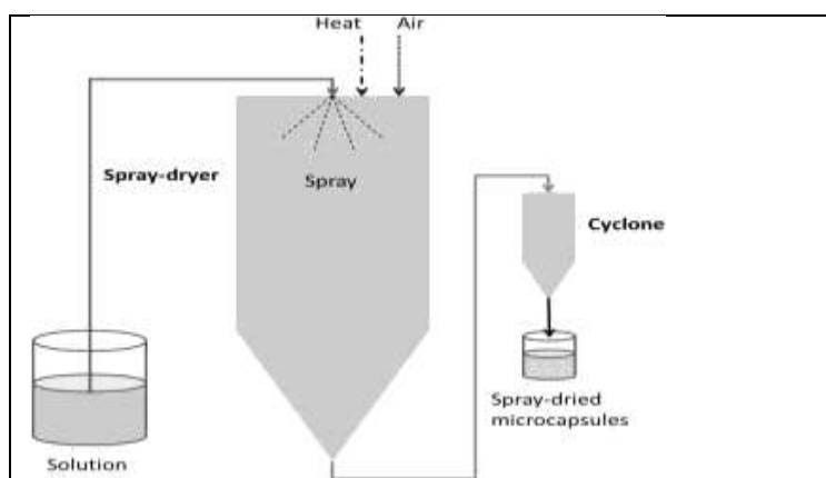
spray drying congealing process
