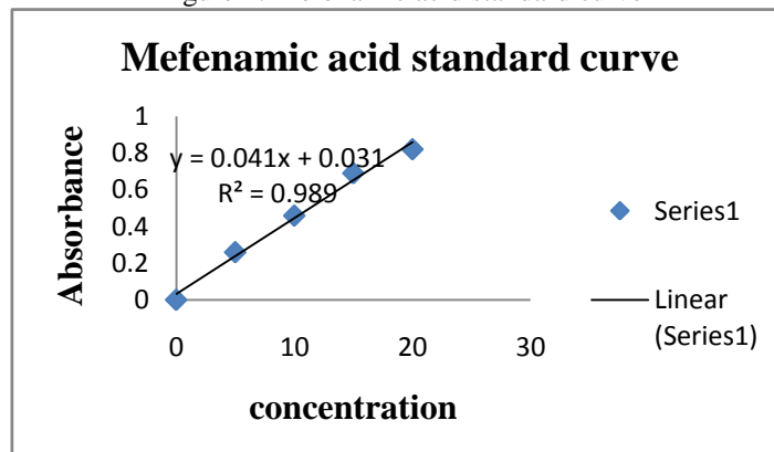
Figure 2: Mefenamic acid standard curve
