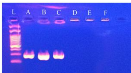
Figure (7): Inhibition studies of prepared compound (Q3) against purified DNA gyrase.
