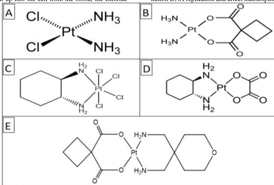
Fig.2 : Molecular Structure of Cisplatin
