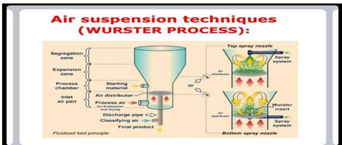
Figure 4 : Air-suspension coating
