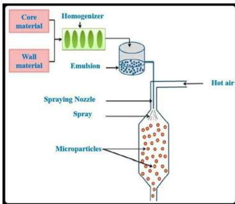
Figure6 : Spray Drying
